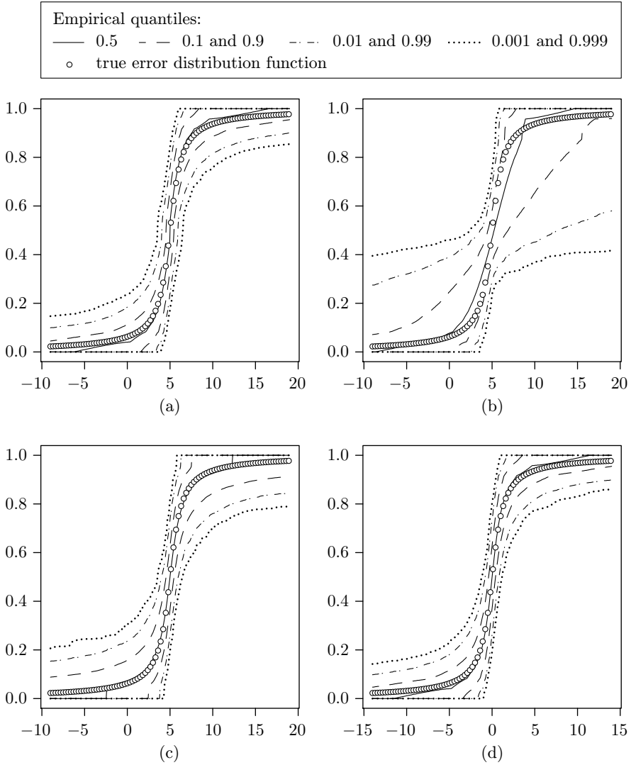
Figure 2. Empirical quantile estimates of the Cauchy distribution function based on (a) \tilde{B} ( \lambda = 0.5 ), (b) \tilde{B} ( \lambda = 0.9 ), (c) \overline{B} , and (d) on the empirical quantile function (EQF) of errors. (Vertical axis: values of the distribution f .)
