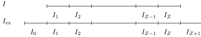
Figure 3. The extended interval I_{\text{ex}} for the case L = R = 1 .
