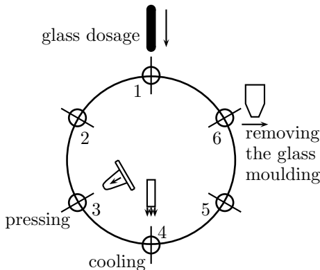
b) Scheme of the carousel press.
