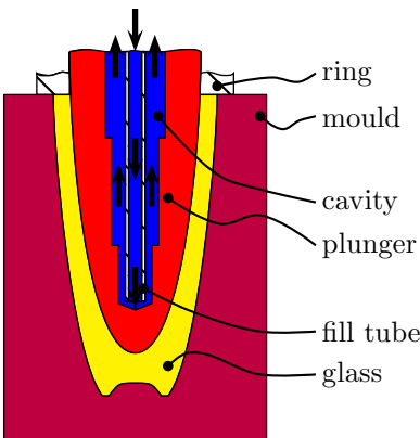
a) Scheme of the system.
