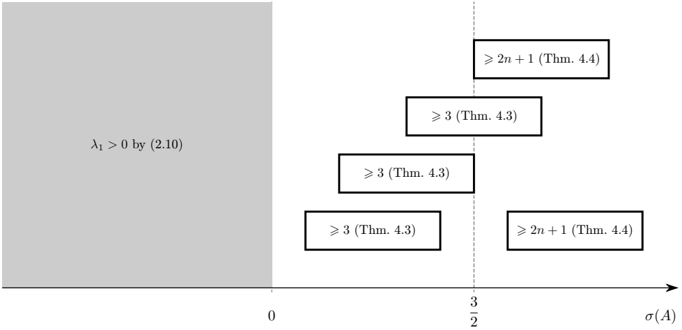
Figure 2. Dependence of number of solutions in the monostable case r < 0 with positive diffusion based on the spectrum \sigma(A) of the matrix A = \frac{1}{2}(1 - hr)I - (\frac{1}{2}hd/\mu^2)L . The picture depicts various positions of \lambda_1 (the left end of the region) and \lambda_N (the right end). Note, that (2.10) implies that the spectrum \sigma(A) is always positive.
